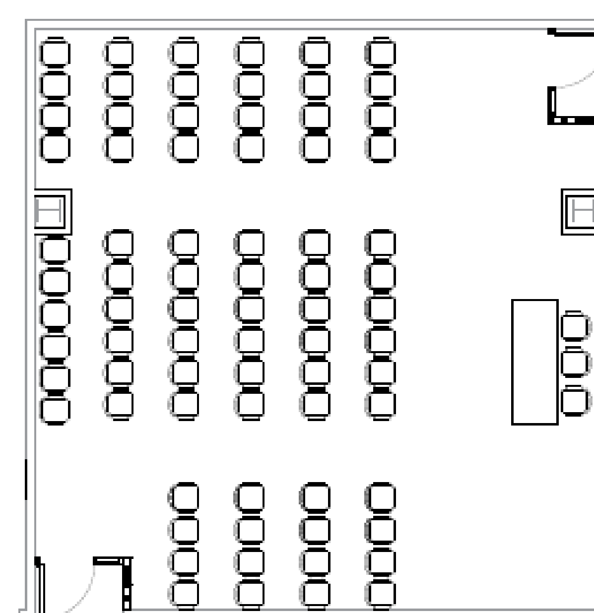
ASSEMBLY LAYOUT
